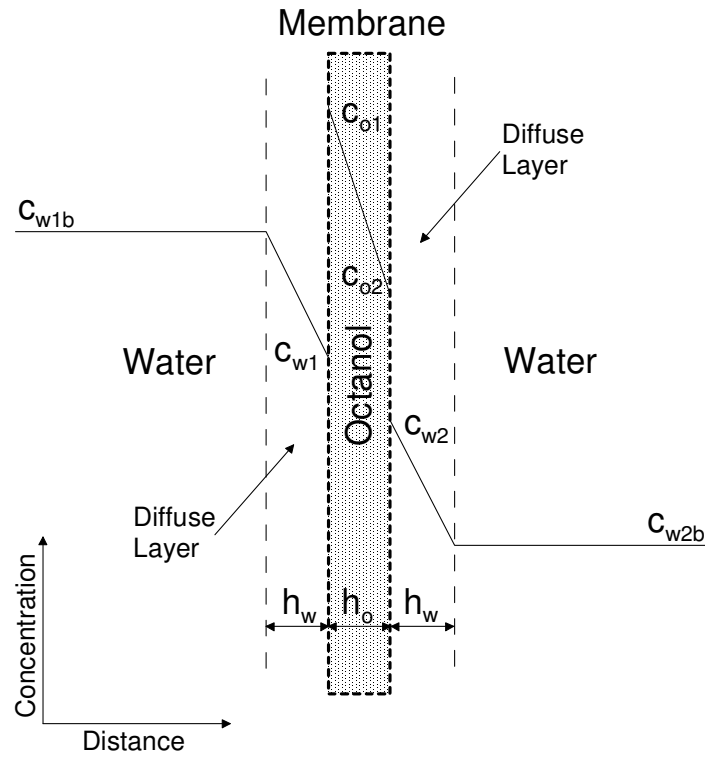
Fig. 1. Two aqueous solutions separated by octanol membrane. Bulk concentrations of substance in two water compartments are denoted by c_{w1b} and c_{w2b} , the concentrations at outer and inner membrane interfaces are denoted by c_{w1} and c_{w2} , and c_{o1} and c_{o2} . h_w is the thickness of diffuse layer in water and h_o the thickness of octanol membrane, which porosity (i.e. fraction of free volume in membrane) is \alpha .
