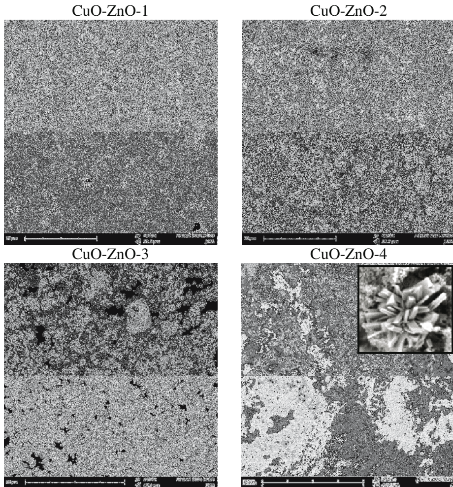
Fig. 4. SEM images of CuO-ZnO samples. Scale bars: 20 \mu\text{m} .
