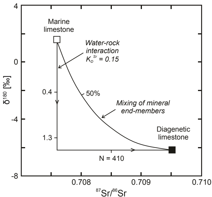
Fig. 8. Modelled oxygen and strontium isotope variations during recrystallization of a marine limestone by freshwater. Water:rock ratios (N) are shown at given stages of the interaction paths. The original limestone is assumed to have \delta^{18}\text{O} = 1.5\text{‰} VPDB, ^{87}\text{Sr}/^{86}\text{Sr} = 0.7076 , C_{\text{Sr}} = 300 ppm, porosity = 20%; the freshwater composition is \delta^{18}\text{O} = -1\text{‰} VSMOW, ^{87}\text{Sr}/^{86}\text{Sr} = 0.7095 , C_{\text{Sr}} = 0.6 ppm. T_{\text{recrystallization}} = 40^\circ\text{C} (after Banner [12]).
