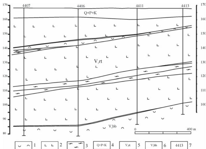
Figure 2. Geological cross section along the line II-II (drillhalls 4407–4413) within the Rafalivka ore district: 1 – tuffs, 2 – basalts, 3 – lavobreccia, 4 – rocks of Creataceous, Paleogene, Quarternary age; 5 – the Ratno Beds; 6 – the Babyno Beds; 7 – drillhore's numbers
