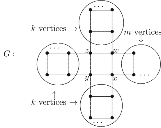
FIGURE 5. Quadrangular outerplanar graph of order n \geq 10 with the path P_4 = xyzw as the union of minimal separators; k, m – even natural numbers such that k > m and n = 3k + m + 4 .
