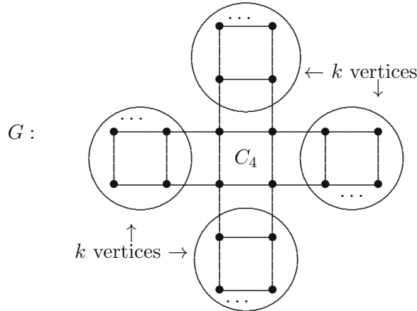
FIGURE 6. Balanced quadrangular outerplanar graph of order n with the cycle C_4 as the union of minimal separators. This structure can be obtained only for n \equiv 4 \pmod 8 ; k = \frac{n-4}{4} .
